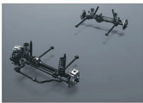
3 LINK RIGID AXLE SUSPENSION
